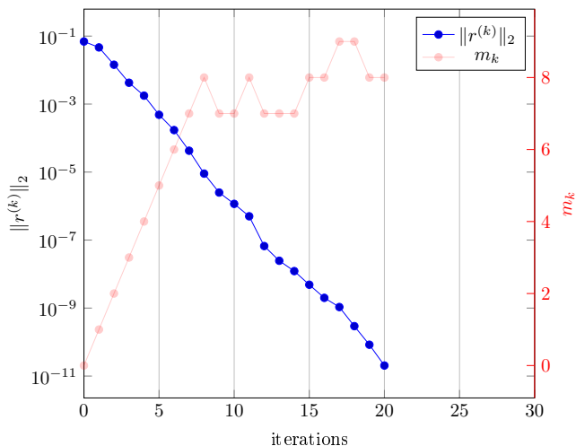
(b) Convergence of the adaptive-depth CDIIS for the dimethylnitramine (RHF-6-31G) molecule with \delta = 0.0001 with the corresponding depth m_k .
