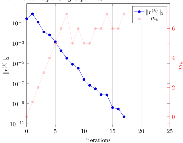
(d) Convergence of the adaptive-depth CDIIS for the glycine (RKS-6-31Gs) molecule with \delta = 0.0001 with the corresponding depth m_k .
