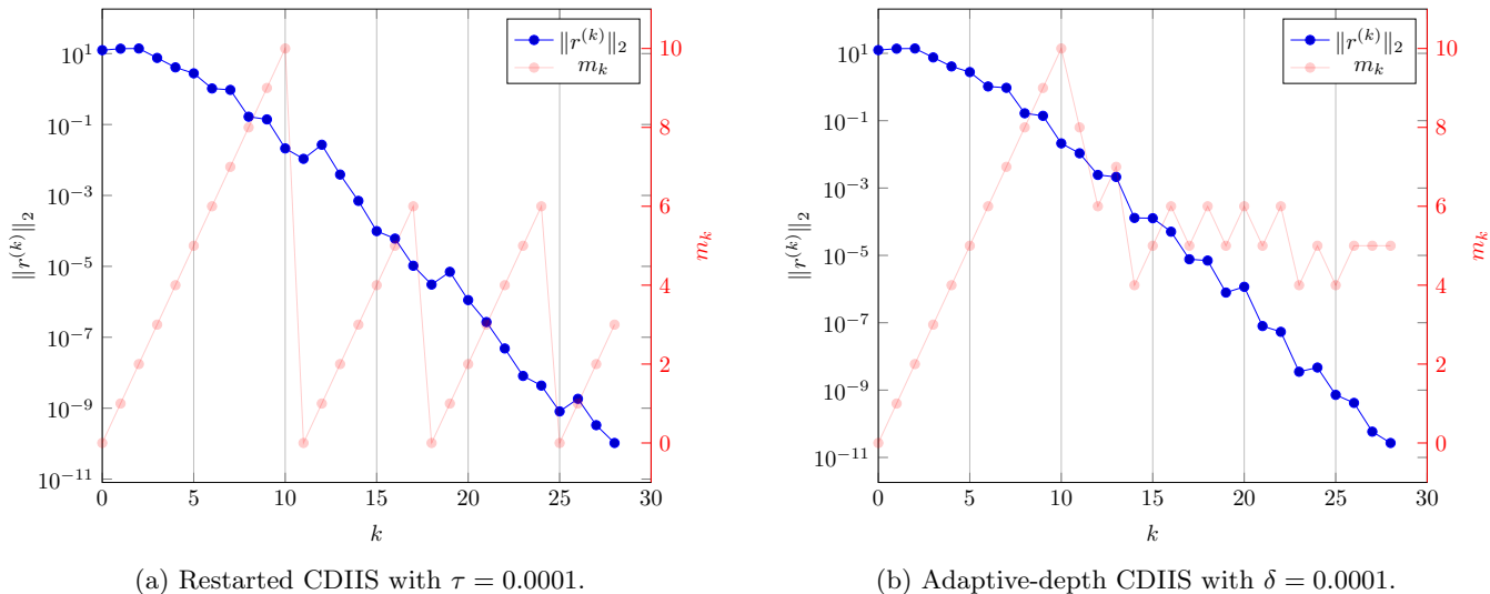
Figure 2: Comparison of the restarted and adaptive-depth CDIIS on the Cadmium-imidazole molecule in the RKS model with basis B3LYP/3-21G.
