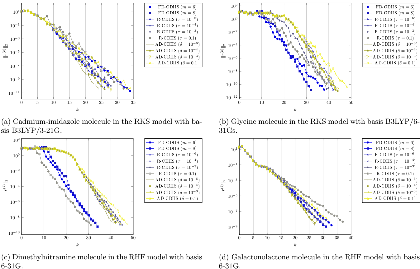
Figure 1: Comparison of the fixed-depth, restarted and adaptive-depth CDHIS on different molecules using initial guess obtained by applying the Aufbau principle to the core Hamiltonian matrix.
