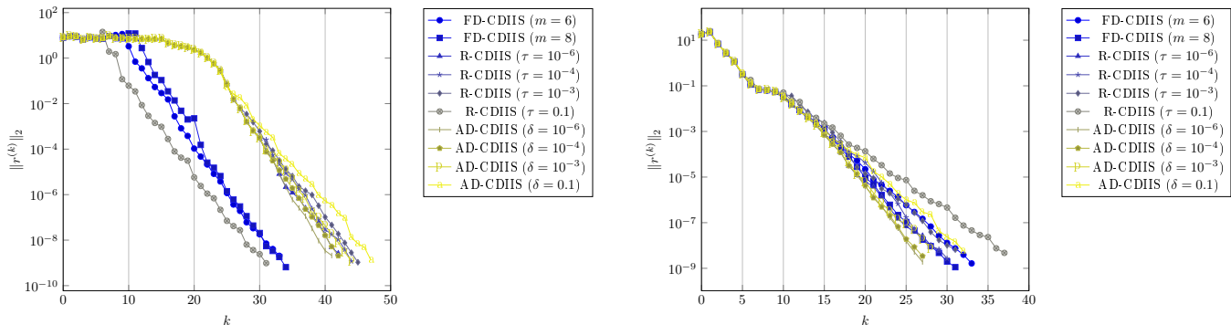
(c) Dimethylnitramine molecule in the RHF model with basis 6-31G.
