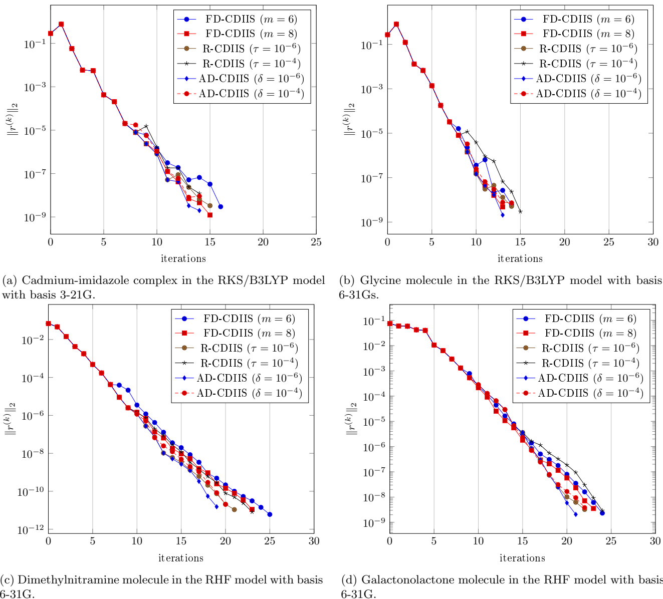
Figure 3: Residual norm convergence for the fixed-depth, restarted and adaptive-depth CDIIS on different molecular systems using an initial guess provided by a globally convergent method.
