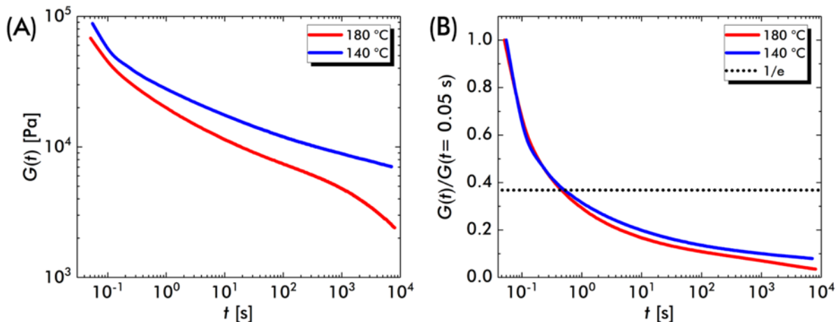
Figure 9. Comparison of PE- \nu stress relaxation data presented in (A) log-log and (B) normalized semi-log formats. The black dashed line in (B) marks when the data decay to a value of 1/e . Data in both panels are the same as those presented in Figure 5B. Panel (B) could suggest that the relaxation time is \sim 0.5 s. This is, however, a gross underestimation, as clearly visible in panel (A). For instance, at 140 °C the stress is not relaxed, even after 8 h.
