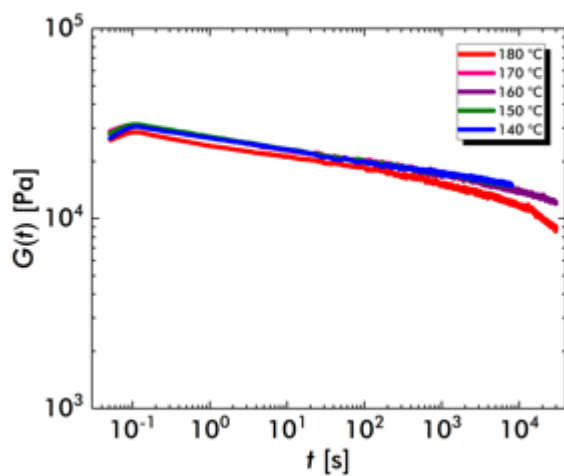
Figure S29. Stress relaxation of PE- v - insol .
