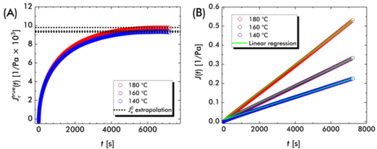
Figure S26. Creep compliance and recovery data for PE- v-sol at varying temperature. (A) Creep recovery. Dotted lines represent the plateau extrapolation used to calculate J_e^0 . (B) Creep compliance. Green lines signify the linear extrapolations used to estimate \eta_0 .
