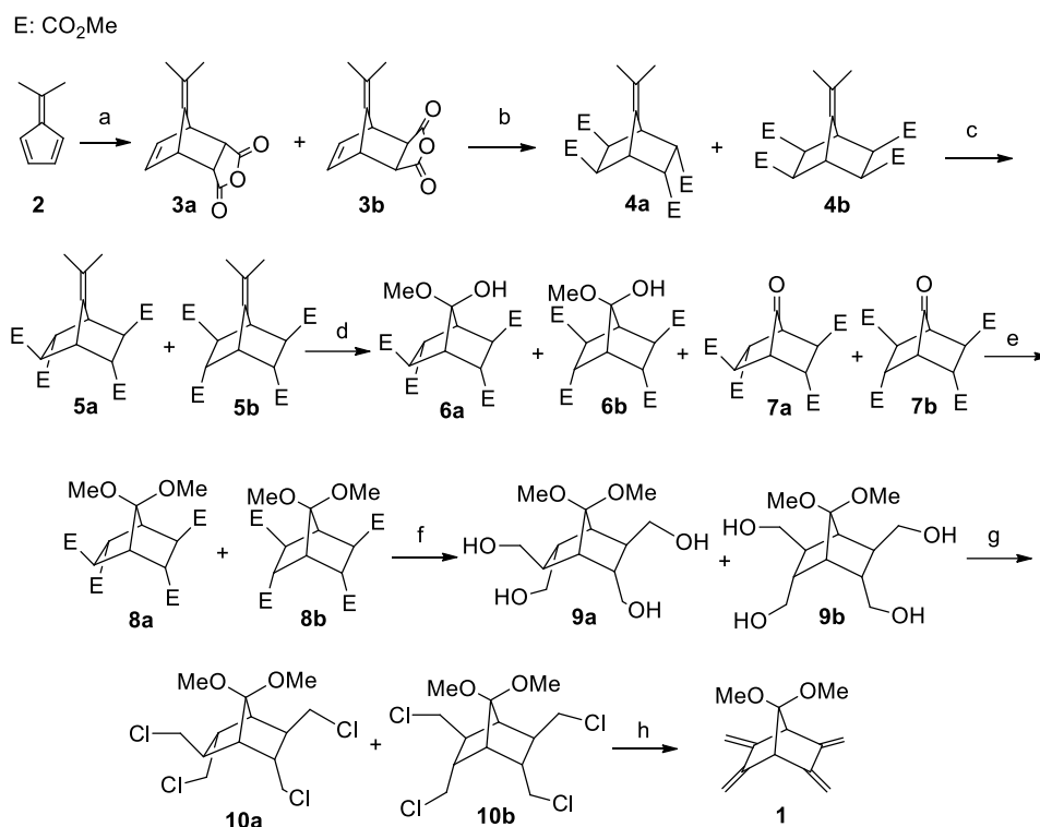
Scheme 2. Synthesis of 1 . a) maleic anhydride, DCM; 86% b) Pd/C, CuCl 2 , CO, MeOH; 74% c) K 2 CO 3 , MeOH; 88% d) O 3 , Me 2 S, DCM-MeOH; e) HC(OMe) 3 , APTS, MeOH; 82% for two steps f) LiAlH 4 , THF; 94% g) Cl 2 , PPh 3 , imidazole, DCM-ACN-pyridine; 68% h) t -BuOK, DMF; 61%.
