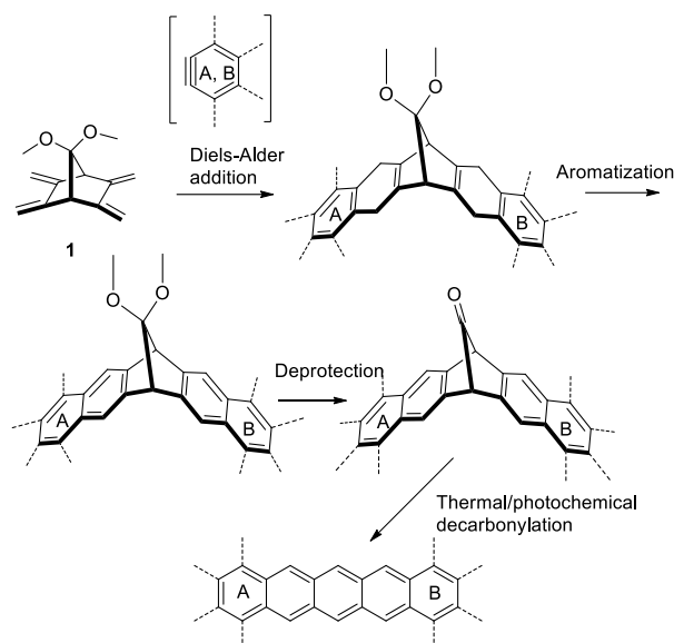
Scheme 1. Preparation of symmetrical ( A=B ) and non-symmetrical ( A\neq B ) acenes by cheletropic decarbonylation of CO bridged precursors.
