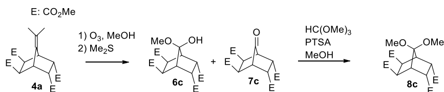
Scheme 3. Ozonolysis of 4a followed by protection of the bridging ketone.
