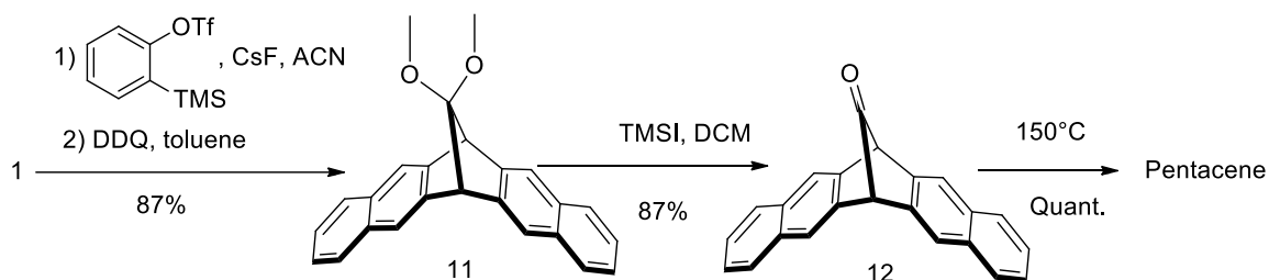
Scheme 4. Preparation of pentacene from 1
