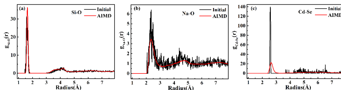
Figure 2. Radial distribution functions for (a) Si–O, (b) Na–O and (c) Cd–Se pairs in the initial structure (black) and averaged over the ab initio molecular dynamics (red), for a quantum dot embedded in the glass matrix.
