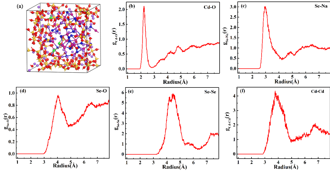
Figure 3. (a) The final configuration from the ab initio molecular dynamics. Radial distribution functions for (b) Cd–O, (c) Se–Na, (d) Se–O, (e) Se–Se, and (f) Cd–Cd pairs, averaged over the ab initio molecular dynamics (red), for a quantum dot embedded in the glass matrix.
