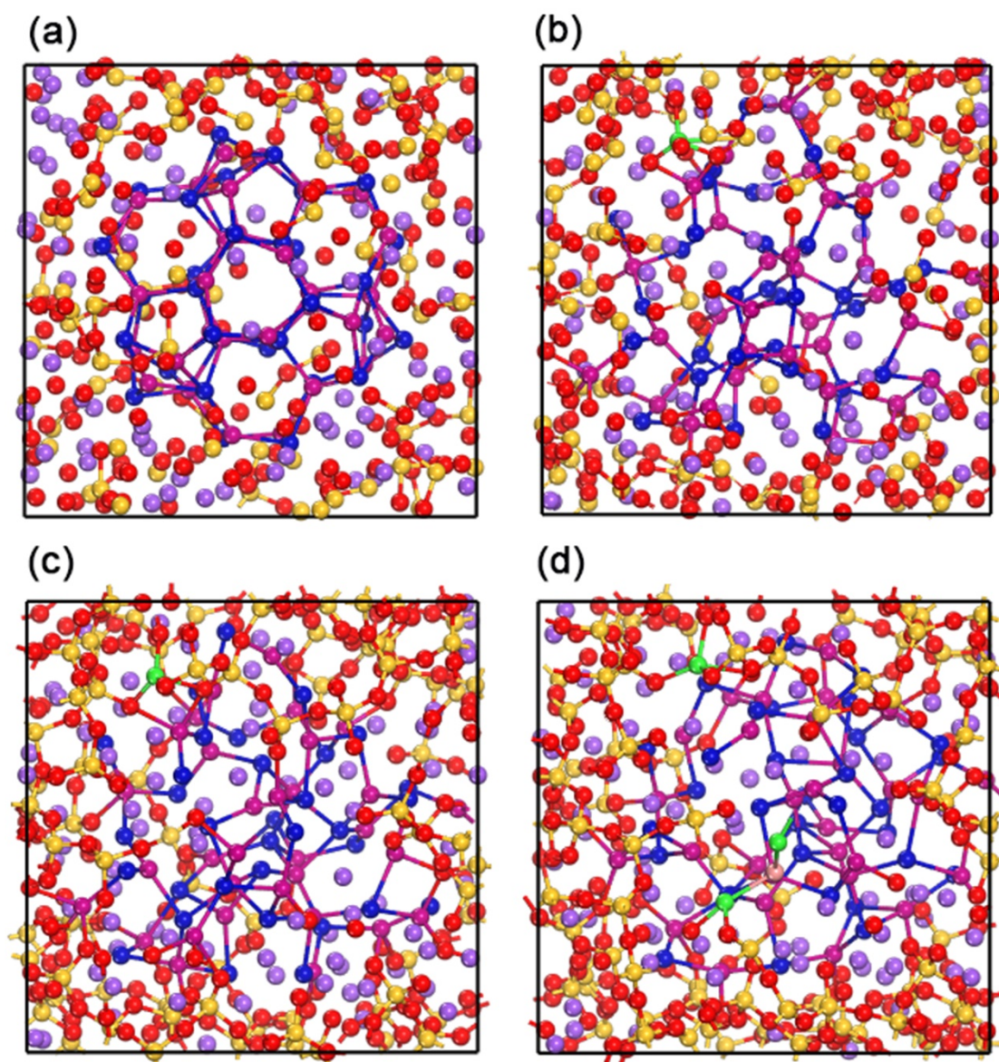
Figure 1. (a) The initial configuration for the classical MD calculations. (b) The final configuration for classical MD simulations, used as initial configuration for the geometry optimization by DFT method. (c) The geometry-optimized structure at the DFT level, used as the initial configuration for the ab initio molecular dynamics. (d) The final configuration from the AIMD simulations. Si: yellow, O: red, Na: purple, Se: magenta, Cd: blue. Se and Cd atoms dissociated from the quantum dot are highlighted in pink and green, respectively.
