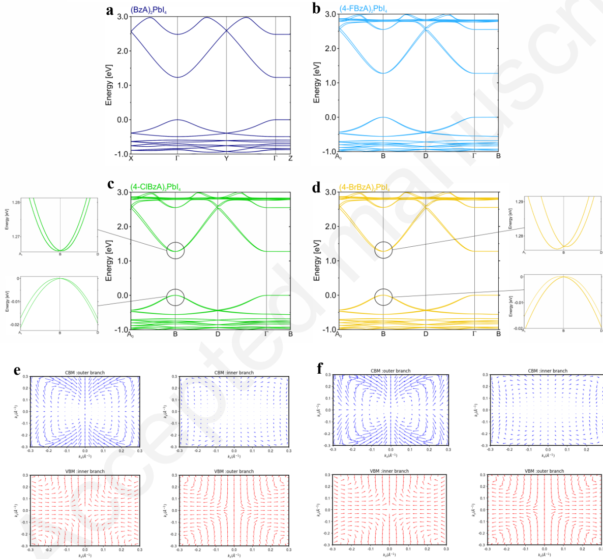
Figure 5. First-principles calculations of electronic band structures of (a) (\text{BzA})_2\text{PbI}_4 , (b) (4\text{-FBzA})_2\text{PbI}_4 , (c) (4\text{-ClBzA})_2\text{PbI}_4 and (d) (4\text{-BrBzA})_2\text{PbI}_4 at 180 K. For (4\text{-ClBzA})_2\text{PbI}_4 and (4\text{-BrBzA})_2\text{PbI}_4 the spin-split band edges are highlighted by zoom-ins. (e-f) spin textures for the inner and outer branches for valence (red) and conduction (blue) bands of (4\text{-ClBzA})_2\text{PbI}_4 and (4\text{-BrBzA})_2\text{PbI}_4 , respectively. The spin textures of both compounds show similar shapes and features, yet with differences in absolute values.
