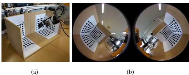
Figure 3. Calibration of the twin-fisheye camera: (a) The calibration rig consists of six checkerboard patterns attached to the inside surface of two half cubes; (b) Sample dual-fisheye image of the calibration rig.
