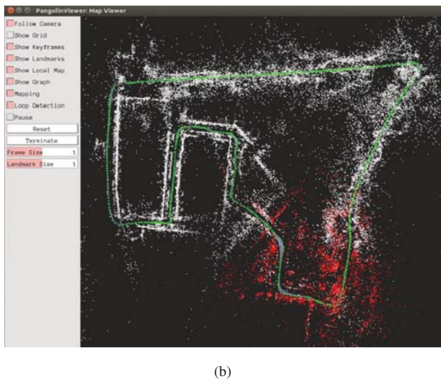
Figure 15. Sequence 7: mapping of the environment: (a) 3-D point cloud obtained by spherical photogrammetry with Agisoft Metashape; (b) 3-D map and robot trajectory (green) obtained with OpenVSLAM (Sumikura et al 2019).
