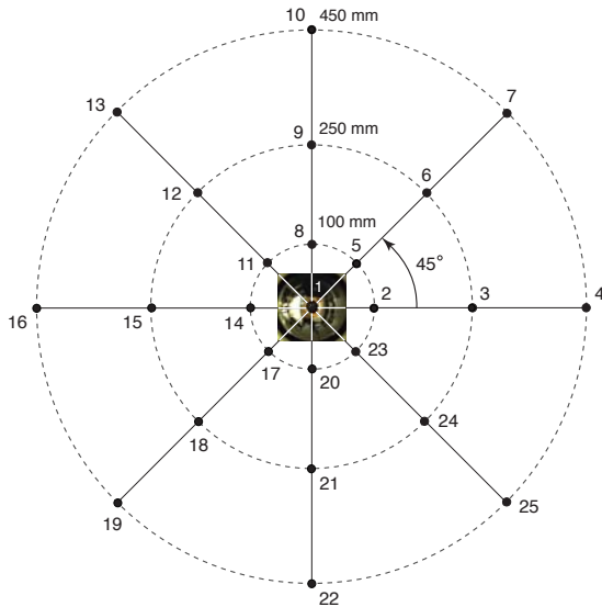
Figure 7. Sequence 1: Graphical illustration of the organization of the images acquired with the catadioptric camera on the Staubli robot: 3600 images were taken at 25 CPs (black disks) lying on 8 rays with an angular spacing of 45^\circ .
