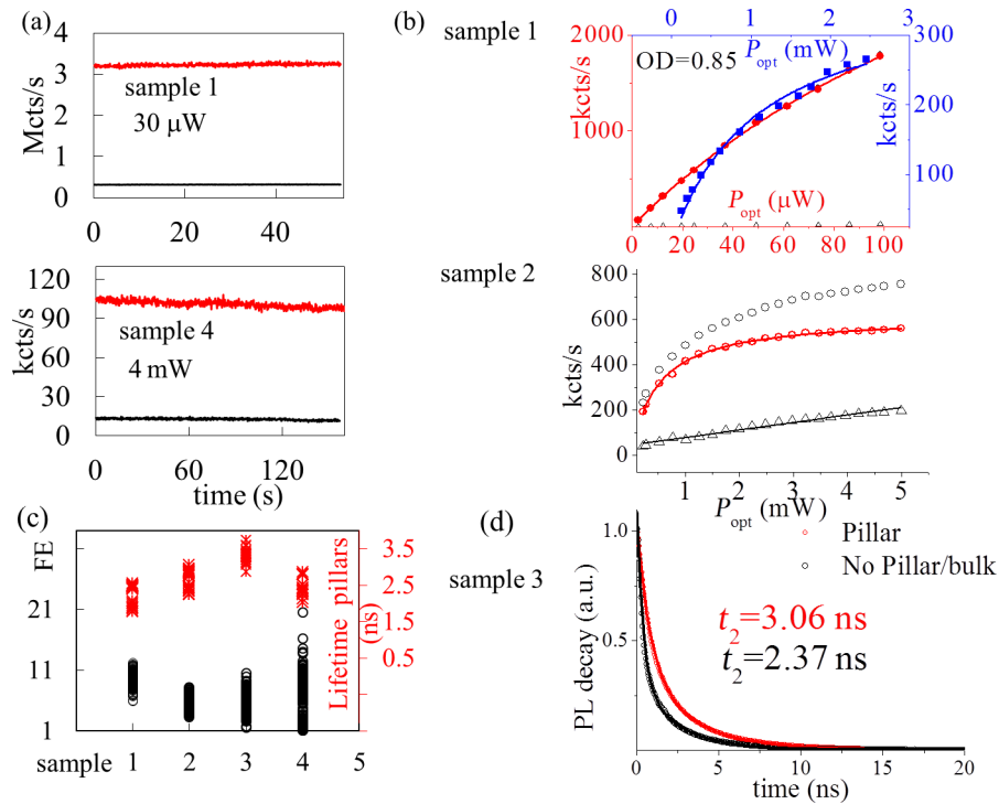
Figure 7: (a) Photostability of one micropillar and the gap region for samples 1 (top) and 4 (bottom) at excitation powers of 30 \mu\text{W} and 4 mW, respectively. Both samples provide a fluorescence enhancement by a factor of about ten. Counts rate are measured every 167 ms. (b) Top: Power saturation curve for one pillar in sample 1 (red) compared with the saturation count rate of the emission in the bulk (blue). The saturation curves show the enhanced emission in the pillar by a factor of 14 and a reduction of the saturation optical power by a factor of 5.6. A neutral density filter with OD = 0.85 was used to perform the measurement. Bottom: Saturation curves for one pillar in sample 2, showing the total count rate, the background, and the signal. (c) Fluorescence enhancement (FE) of more than 100 pillars in different samples (circles) and related lifetime of the emitters in different nanopillars of the four samples. (d) Example of lifetime measurements for V_{\text{Si}} in the pillar and in the gap for sample 3, two exponential decays were observed, the long component of the lifetime is shown. The ratio of the lifetime between the emitters in the bulk and in the pillar (for the longest pillar lifetime measured), \tau_{\text{bulk}}/\tau_{\text{pillar}} , is 0.77.
