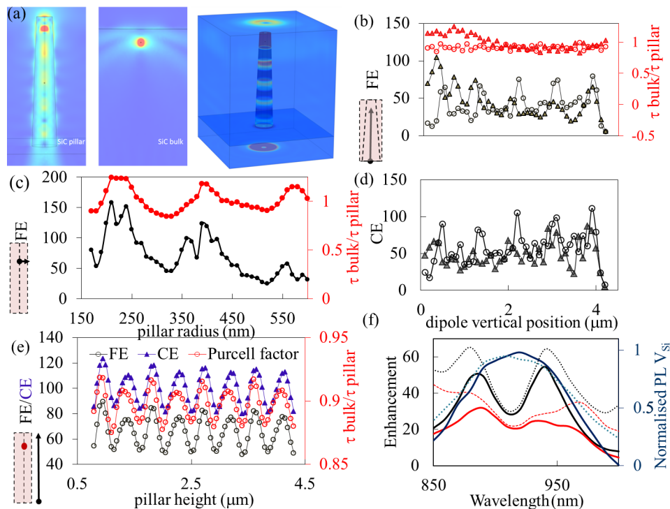
Figure 8: Finite-element method simulation for a pillar of 4.3 \mu\text{m} height and a dipole orientation 8^\circ off the c -axis. Two geometries of the pillars are considered, cylindrical (circles) and conical (triangles). (a) Radiation pattern: intensity and power outflow from a conical pillar with emitters at 3.9 \mu\text{m} from the bottom of a pillar, compared to an emitter 400 nm below the bulk surface. (b) FE and \tau_{\text{bulk}}/\tau_{\text{pillar}} as functions of the vertical position of the dipole for a cylindrical pillar of radius 350 nm (circles) and for the conical pillar (triangles). (c) FE and \tau_{\text{bulk}}/\tau_{\text{pillar}} as functions of the radius of a cylindrical SiC pillar for a dipole located at 3.9 \mu\text{m} from the bottom. (d) Simulated collection efficiency (CE) enhancement relative to bulk as a function of the vertical position of the dipole in a cylindrical pillar of radius 350 nm (circles) and for the conical pillar (triangles). (e) FE, CE, and Purcell factor as functions of the pillar height of the conical pillar with a fixed emitter at 450 nm from the surface. (f) FE (red lines) and CE (black lines) enhancement as functions of the wavelength for the conical pillar with an emitter located at 2.3 \mu\text{m} from the bottom (experimental case), showing the effect of the broad emission of V_{\text{Si}} on FE and CE. The FE reduction across the spectra is ca. 24% compared to a narrow emission. Dashed lines represent the calculated enhancements, and the solid lines represent the enhancement modulated by the emission spectra of V_{\text{Si}} , which is also shown as a dashed blue line in the bulk and solid blue line in the pillar.
