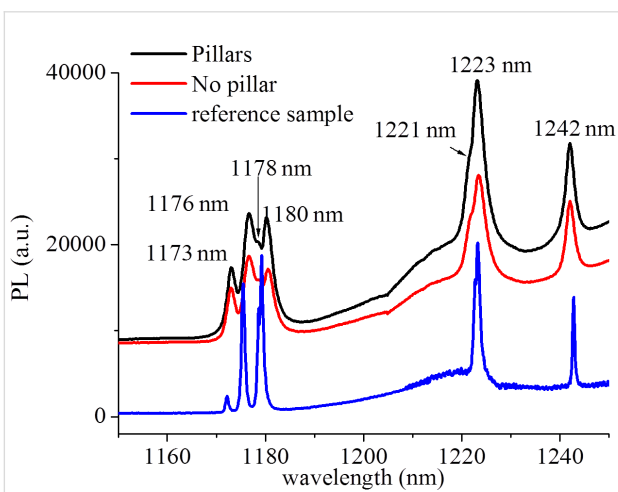
Figure 3: PL emission of sample 3 after excitation at 940 nm at 12 K, showing ZPL emissions at 1221, 1223, and 1242 nm [35,38,39] attributed to NV in 4H-SiC in the micropillars in addition to the ZPLs of the divacancy [34]. The ZPLs from 1173–1180 nm are due to V_C V_{Si} . The spectrum referred to as reference sample was characterized in [38,39] and is given here to prove the emission is indeed due to NV in 4H-SiC.
