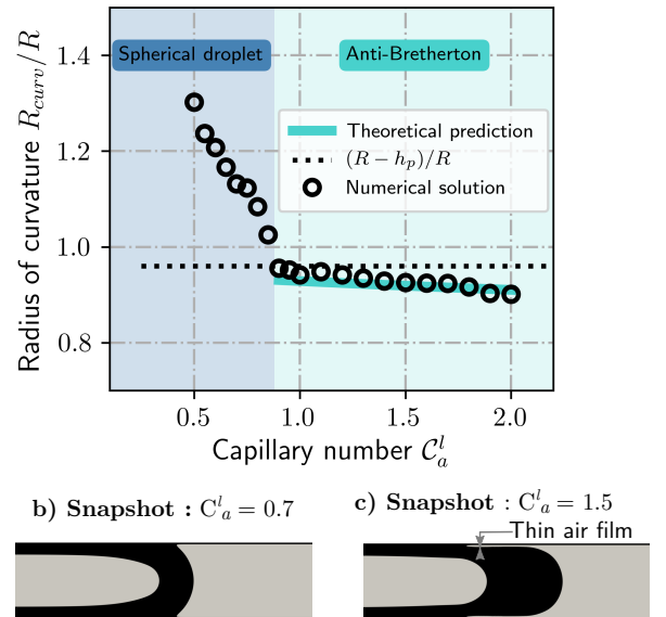
FIG. 2: (a) Numerical evaluation of the front interface curvature R_{curv} of the front interface of a liquid plug divided by the tube radius R as a function of the capillary number C_a^l (at constant Ohnesorge number \mathcal{O}_h = 0.4 ). When the radius of curvature exceeds the tube radius (snapshot (b)), spherical droplets are formed when the plug ruptures. When it becomes smaller than the tube radius (above a critical capillary number), a thin film of air appears between the plug and the walls (snapshot (c)) leading to the formation of an anti-Bretherton drop. (b) Snapshot of numerical simulation: C_a^l = 0.7 , \mathcal{O}_h = 0.4 (c) Snapshot of numerical simulation: C_a^l = 1.5 , \mathcal{O}_h = 0.4
