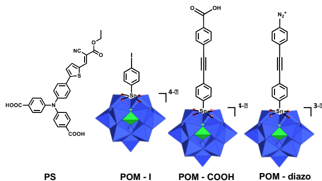
Figure 1. From left to right, drawing of the push-pull organic dye and polyhedral representation of [PW_{11}O_{39}\{SnC_6H_4I\}]^{4-} ( POM-I ), [PW_{11}O_{39}\{SnC_6H_4-COOH\}]^{4-} ( POM-COOH ) and [PW_{11}O_{39}\{SnC_6H_4-N_2^+\}]^{3-} ( POM-diazo ); the WO_6 octahedra are depicted with oxygen atoms at the vertices and metal cations buried inside. Color code: WO_6 octahedra, blue; PO_4 tetrahedra, green.
