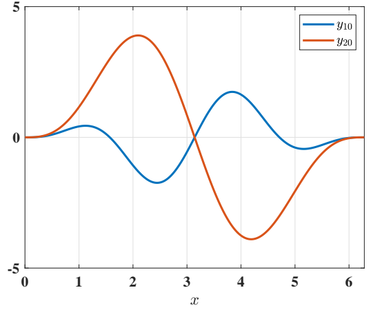
Fig. 4. Initial data of y_1 and y_2 .
