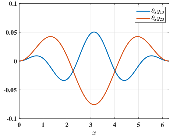
Fig. 5. Initial data of \partial_x y_1 and \partial_x y_2 .
