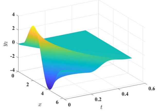
Fig. 3. Response of state y_2 .
