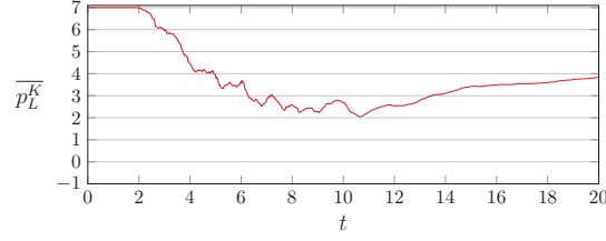
FIGURE 5. TGV at Re = 5,000 : evolution of the average scale-partition parameter for \sigma_{th} = 0.18 and \beta = 0.7 .
