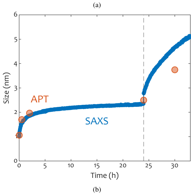
Figure 2: (a) Zn-Zn pair correlation functions (PCF) obtained by APT on a model Al-Zn-Mg-Cu alloys for different ageing times (circles) along with the fits from the method in [17]. Both the amplitudes and correlation lengths increase with ageing times. (b) Size of the precipitates obtained by in situ SAXS (blue dots) and ex situ APT (red circles). The agreement is very good.
