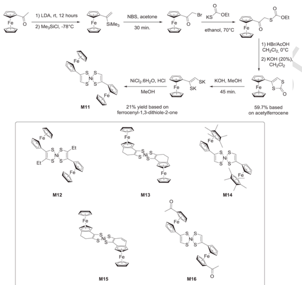
Fig. 37. Synthetic route to dithiolenes-containing metal complexes M11 and chemical structures of M12-M16 .
