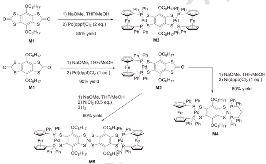
Fig. 33. Synthetic route to dithiolenes-containing metal complexes M2, M3, M4 and M5.
