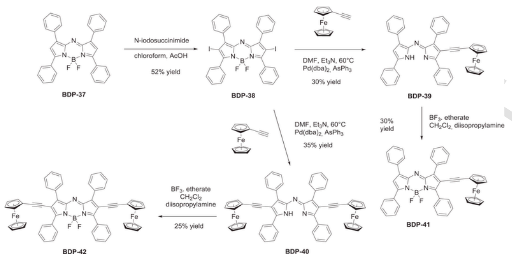
Fig. 14. Synthetic route to BDP-41 and BDP-42.
