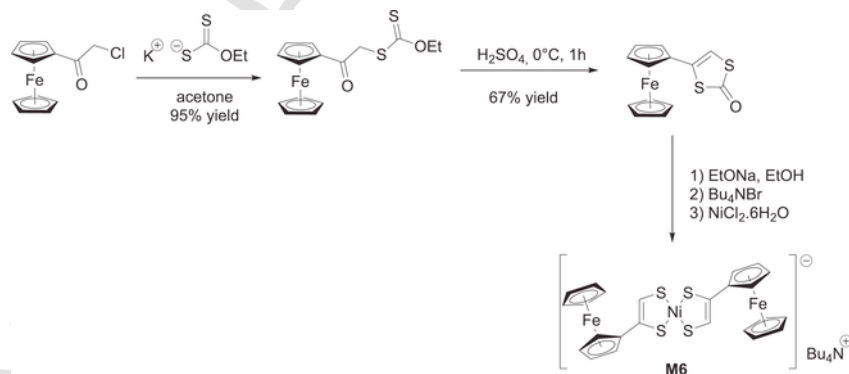
Fig. 34. Synthetic route to dithiolenes-containing metal complex M6.
