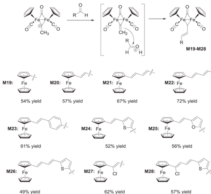
Fig. 39. Synthetic route to metalloenes M19-M28.
