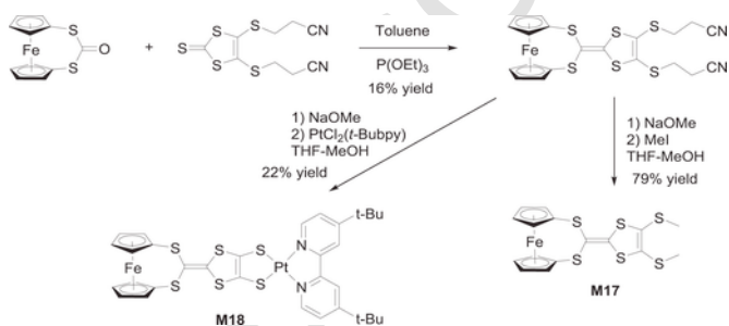
Fig. 38. Synthetic route to dithiolenes-containing metal complexes M17 and M18 .
