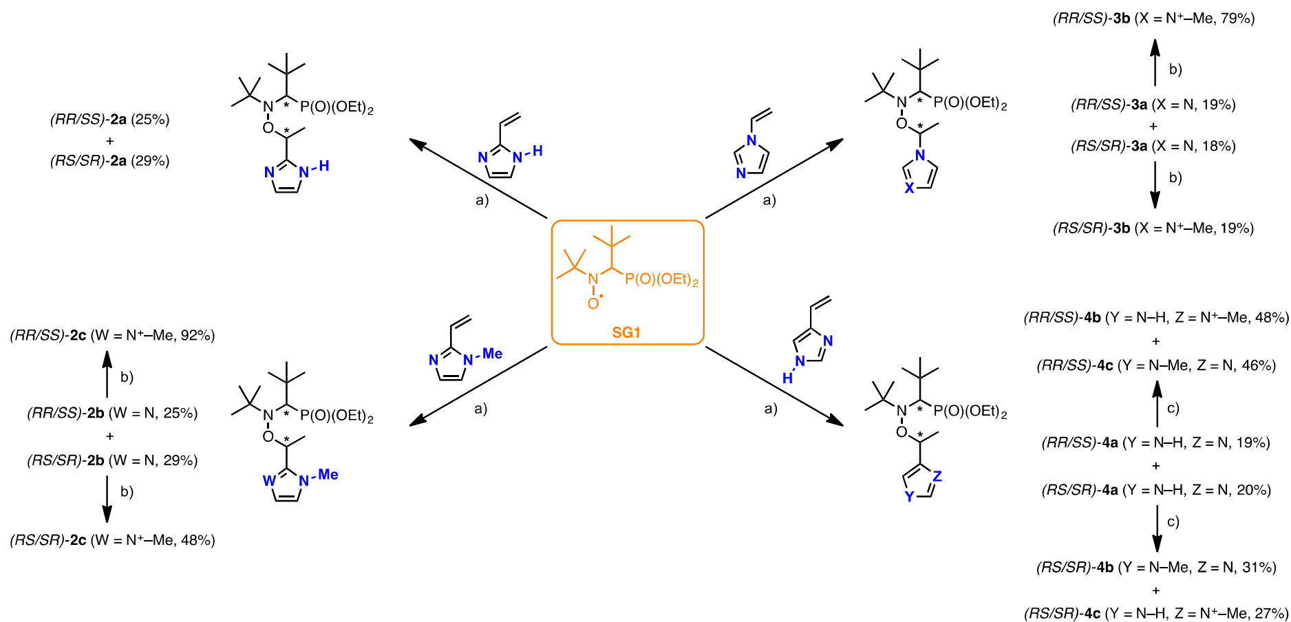
Scheme 2 Synthesis of alkoxyamines (RR/SS)\text{-} and (RS/SR)\text{-} 2a-c , 3a-b , 4a-c : a) \text{MnCl}_2 , N,N' -bis(salicylidene)ethylenediamine (salen), \text{NaBH}_4 , i\text{-PrOH} , air; b) methyl p -toluenesulfonate, THF; c) \text{MeI} , \text{K}_2\text{CO}_3 , \text{CH}_2\text{Cl}_2 .
