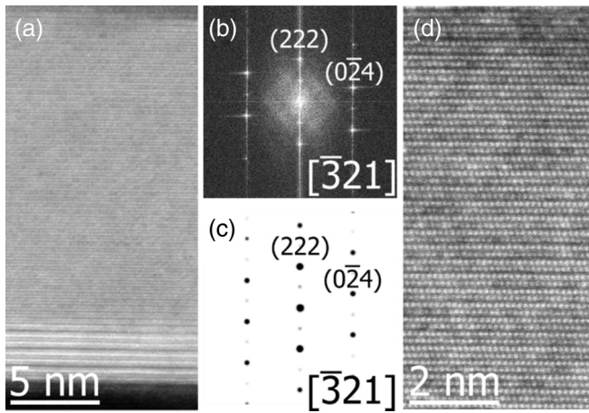
FIG. 2. HAADF image of (a) SnTe film along the [321] zone axis with corresponding (b) fast Fourier transform and (c) simulated diffraction pattern of SnTe along the same zone axis. (d) High-resolution HAADF-STEM image of SnTe film. The layered structure at the bottom of the film in (a) consists of three QLs of \text{Bi}_2\text{Te}_3 buffer.
