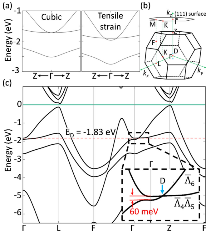
FIG. 5. (a) The evolution of the band structure under out-of-plane tensile strain along the [111] direction along the Z- \Gamma -Z direction of (b) the Brillouin zone. Note that Z and L points become equivalent in the unstrained cubic case. (c) Band structure of bulk out-of-plane tensile strained SnTe along the \Gamma -L-F- \Gamma -Z-F direction of the Brillouin zone. The inset shows a magnification around the Dirac point D marked by the blue vertical arrow.
