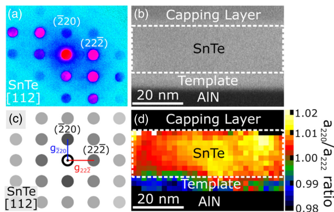
FIG. 3. (a) NPED pattern from the SnTe layer along the [112] zone axis. (b) STEM image of the region analyzed with NPED. (c) Simulated NPED pattern along [112] showing the in-plane reflections (\bar{2}20) and out-of-plane (22\bar{2}) reflections which were used to determine the ratio of lattice parameter r = (\alpha_{\bar{2}20})/\alpha_{22\bar{2}} . (d) Map of the r ratio in the SnTe region (dashed box), where each pixel corresponds to a NPED pattern.
