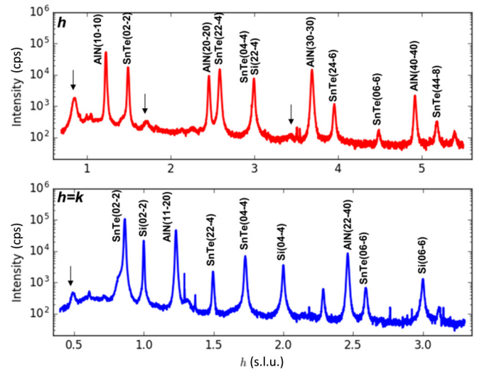
FIG. 4. Radial scans along the in-plane h and h = k directions as a function of the \text{Si}(111) surface reciprocal-lattice units. Each peak has been indexed according to International Centre for Diffraction Data database files using cubic (SnTe, Si) and hexagonal (AlN) Miller index notations. Arrows point out peaks which are not Bragg peaks but overlayer SnTe crystal truncation rod signals. The peak patterns in h and h = k directions are compatible with the presence of 30^\circ rotated domains.
