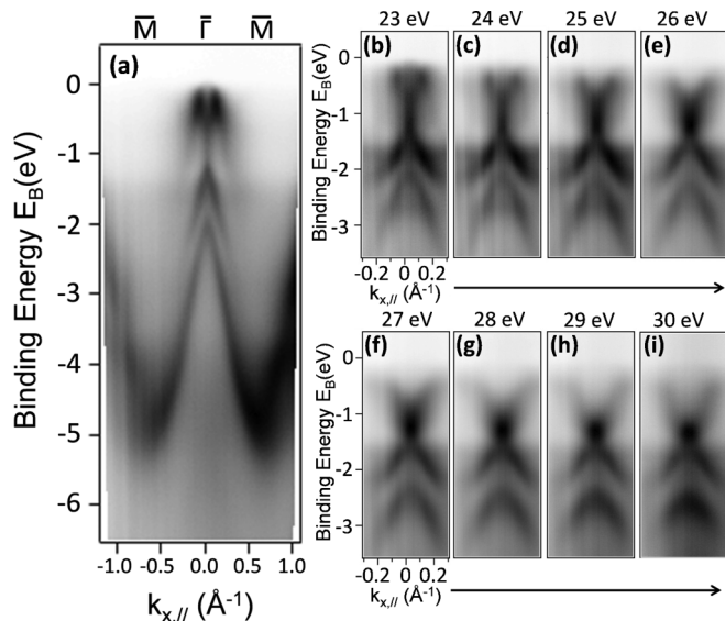
FIG. 7. (a) Energy dispersion along the \bar{M}\bar{\Gamma}\bar{M} direction of the Brillouin zone taken with photon energy h\nu = 65 eV and (b)–(i) ARPES of SnTe taken at different photon energies h\nu from 23 to 30 eV.
