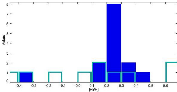
Fig. 4. Distribution of [Fe/H] of the stars observed in the field of Be 81. The cyan rectangles show the GIRAFFE metallicities of RV member stars, while the blue ones indicate the UVES metallicities (including star 19015978-0028183).
