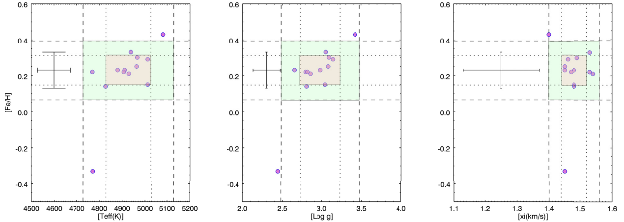
Fig. 3. [Fe/H] vs. atmospheric parameters of UVES stars in Be 81. The dotted lines mark the 1\sigma region, while the dashed lines indicate the 2\sigma area. The typical error bar on each star are shown on the left side of each panel.
