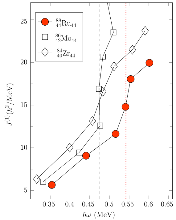
FIG. 2. Experimental values for the kinematical moment of inertia ( J^{(1)} ) for the low-lying yrast bands of the N = 44 isotones ^{88}\text{Ru}_{44} (this work), ^{86}\text{Mo}_{44} [40,41], and ^{84}\text{Zr}_{44} [42]. The black dashed vertical line indicates the approximate rotational frequency of the first isovector-paired band crossing due to g_{9/2} protons as predicted by standard cranked shell model calculations [43,44]. The red dotted vertical line indicates the band crossing frequency for the ground-state band in ^{88}\text{Ru}_{44} observed in this work.
