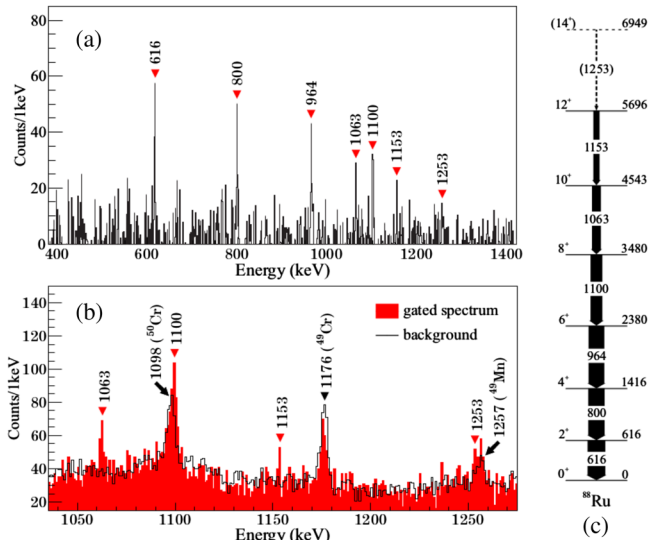
FIG. 1. (a) Gamma-ray energy spectrum detected in coincidence with the 616, 800, 964, and 1100 keV \gamma rays, with the additional requirement that two neutrons and no charged particles were detected in coincidence. (b) Expanded part of the unsubtracted gated spectrum around the new \gamma -ray transitions at 1063 keV ( 10^+ \rightarrow 8^+ ), 1153 keV ( 12^+ \rightarrow 10^+ ), and 1253 keV [ (14^+) \rightarrow 12^+ ] is drawn in red together with the background spectrum (black) used to produce the spectrum shown in (a). Gamma-ray peaks due to contaminant reactions on oxygen leading to the population of excited states in ^{49,50}\text{Cr} and ^{49}\text{Mn} are indicated. (c) Level scheme of ^{88}\text{Ru} deduced from the present work. Relative intensities are proportional to the widths of the arrows.
