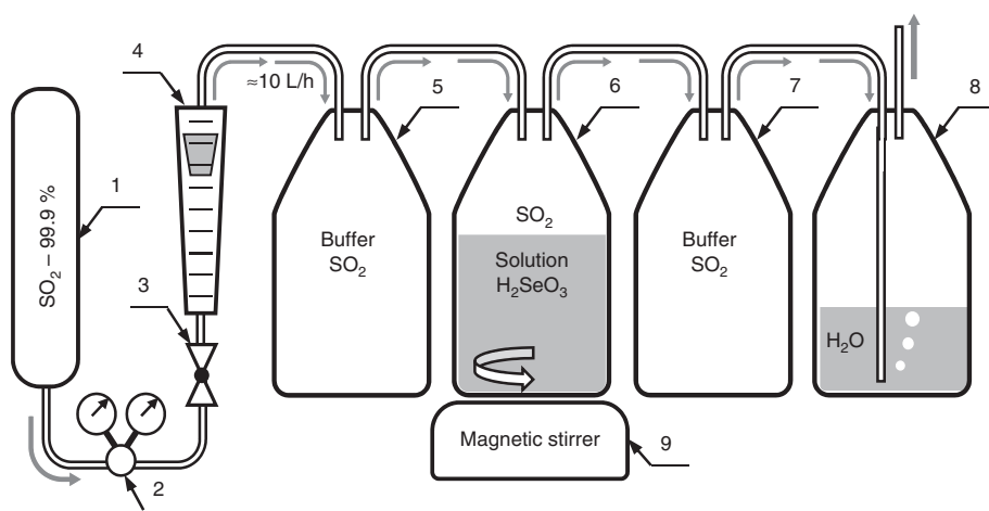
Figure 2: The Scheme for the reduction system of selenious acid (H 2 SeO 3 ) to an elemental state (Se). 1 – a cylinder with SO 2 , 2 – a reducer, 3 – a control valve, 4 – a rotameter, 5–8 – polypropylene vessels (10 L), 9 – a magnetic stirrer.
