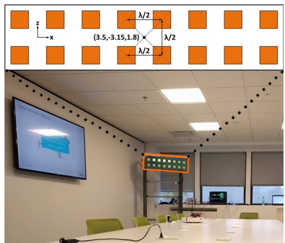
Fig. 1: Environmental setup [7].
