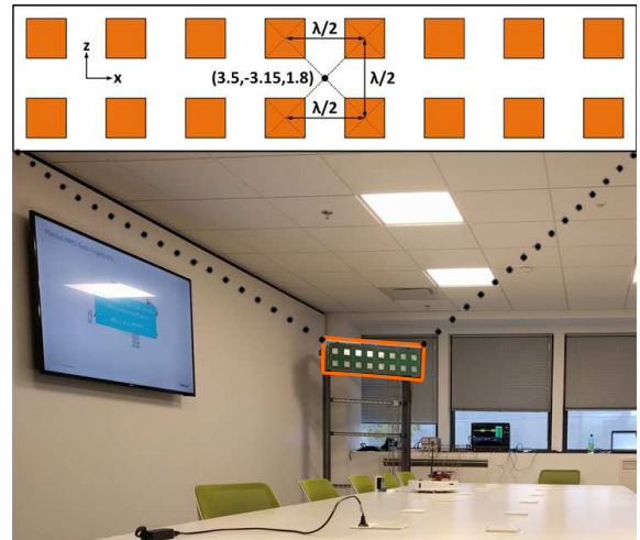
Fig. 1: Environmental setup [7].
