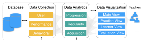
Figure 5: An overview of the architecture of PROGDASH.
