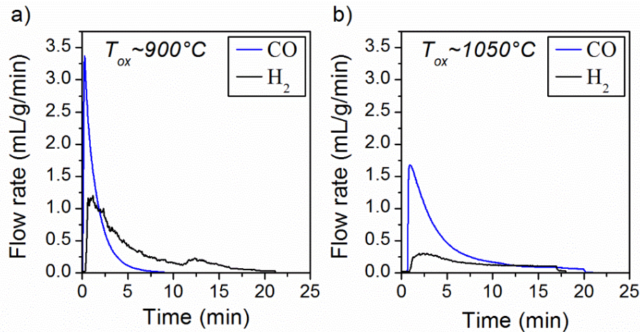
Figure 8: Evolution of H 2 and CO production rates with an oxidation temperature of a) 900°C (cycles #6 and #7 of CF-20) and b) 1050°C (cycles #5 and #9 of CF-20).
