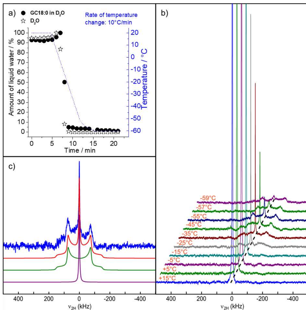
Figure S 5: ^2\text{H} solid-state NMR experiments performed during freezing from +20^\circ\text{C} to -60^\circ\text{C} at a rate of 10^\circ\text{C}\cdot\text{min}^{-1} for a GC18:0 lamellar hydrogel ( C = 5 \text{ wt}\% , \text{pH} = 6.2 \pm 0.3 , [\text{NaCl}] = 300 \text{ mM} ) prepared in 100% \text{D}_2\text{O} . Temperature is controlled directly in the NMR probe using the BCU-Xtreme temperature unit. The sample is placed in a typical zirconia 4 mm-rotor and the temperature is measured outside the rotor. a) Evolution of the amount of liquid water in the lamellar hydrogel (circles, left) and in pure \text{D}_2\text{O} (stars, left) and corresponding temperature profile (dashed line, right). The amount represents the normalized integrals of the resonance at 0 kHz (Lorentzian component corresponding to liquid-like water) of the ^2\text{H} -NMR spectra. A slight increase of the measured amount of liquid water was observed before freezing. This could be explained by a faster longitudinal T_1 relaxation rate when decreasing temperature and mobility, favoring quantification. b) Selected ^2\text{H} -NMR spectra of the lamellar hydrogel and relative averaged temperature corresponding to the data in a); a dashed line guides the eye to follow the central resonance at
