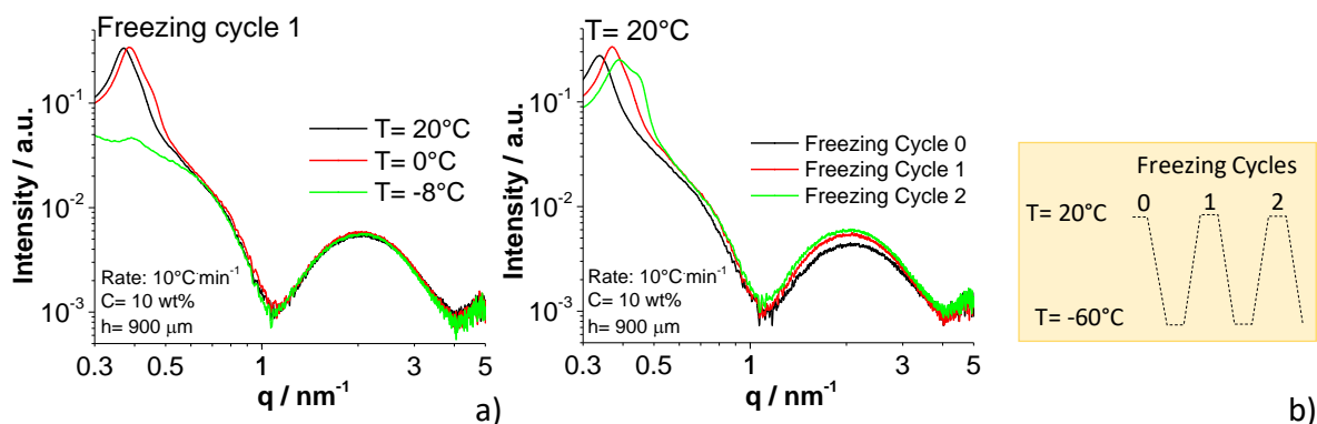
Figure S 3: Background-subtracted SAXS profiles recorded on a GC18:0 lamellar hydrogel ( C = 10 \text{ wt}\% , \text{pH} = 6.2 \pm 0.3 , [\text{NaCl}] = 50 \text{ mM} ) in the ice-templating device shown in Figure S 1 at freezing rate of
