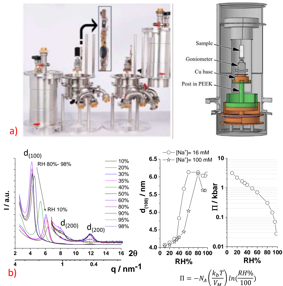
Figure S 4: a) Humidity chamber used on the D16 beamline at ILL and used to perform adiabatic desiccation experiments. 7 b) Evolution of the diffraction patterns as a function of relative humidity, RH\% , measured on a GC18:0 solution (bulk data: C= 1 \text{ wt}\% , \text{pH } 6.2 \pm 0.3 , [\text{NaCl}]= 16 \text{ mM} ) drop-cast on a silicon (111) substrate. Evolution of the d_{(100)} -spacing with RH\% , and plot of the corresponding \Pi(RH\%) relationship with N_A being the Avogadro's number, K_b the Boltzmann constant, T the temperature in Kelvin degrees and V_m the water molar volume.
