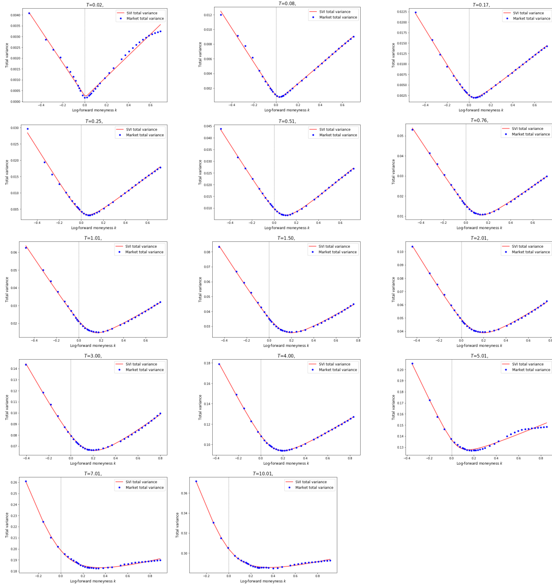
Figure 4.7: Plots of the SVI fits to the call Euro Stoxx 50 implied volatilities for each of the 14th listed starting on April 05, 2019.
