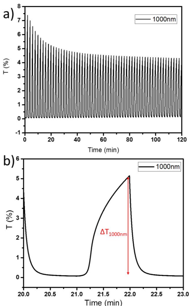
Figure 8. In-situ transmittance curves of the WO_3/LiTFSI in EMITFSI/Pt vs SCE recorded at 1000 nm with voltammetry cyclic range from -1 V to +1 V: (a) 60 cycles, (b) focus on one single cycle. WO_3 films were doctor bladed from the raw powder.
