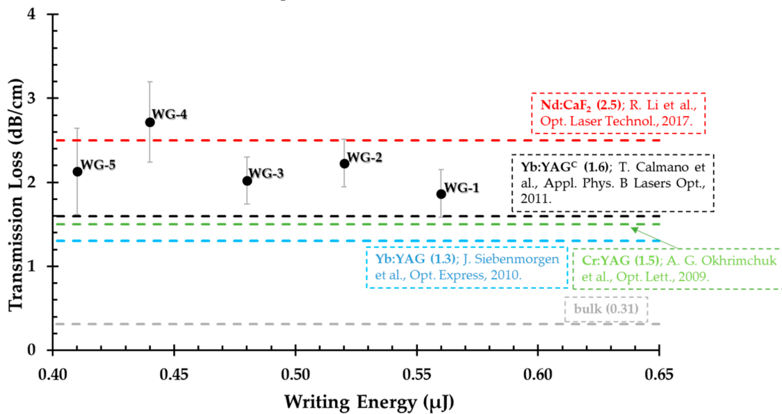
Figure 4. Transmission loss (dB/cm) of the \text{CaF}_2 undoped crystal double-track waveguides in comparison with some previously reported transmission losses where red is for a Nd:CaF 2 crystal [31]; black for a Yb:YAG ceramic [49]; green for a Cr:YAG crystal [17] and blue for a Yb:YAG crystal [11]. The gray line at 0.31 dB/cm is the transmission loss of the \text{CaF}_2 unmodified zone. The error bars in the measurements indicate the standard deviation of the data from multiple experimental runs.
