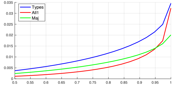
Fig. 2. V as a function of correlation c , d = 256 , n = 15 .
