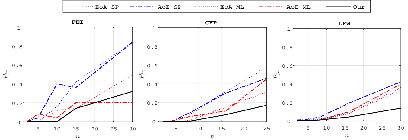
Fig. 3. Verification performance P_{fn}@P_{fp} = 0.05 vs. group size n for the baselines (see Sect. ??) and our scheme.
