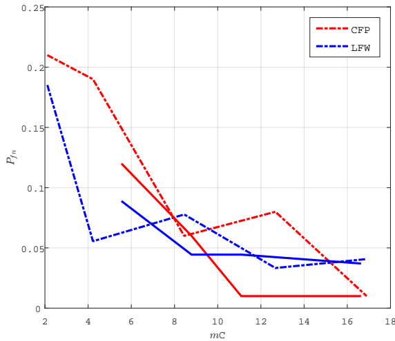
Fig. 4. Verification performance P_{in} @ P_{fp} = 0.05 vs. mC , for n = 16 . This quantity is reduced by decreasing m (dashed lines) or by decreasing C thanks to a surjection (solid lines).
