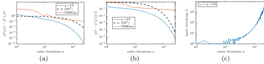
Fig. 3 Inexact primal-dual on the smoothed \text{TV-}L^2 problem. (a) and (b) loglog plots of the relative objective error respectively relative error in norm vs. the outer iteration numbers for accelerated primal-dual (PDHGacc) and inexact primal-dual (iPD) for q = 0.9 , (c) loglog plot of the inner iteration number vs. outer iteration number for q = 0.9 . One can observe that the predicted convergence rate of O(\theta^N) is exactly attained, while for lower outer iteration numbers the necessary amount of inner iterations stays reasonably low.
