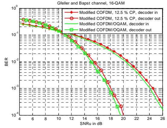
Figure 6. 16-QAM modified schemes over Gfeller & Bapst channel.
