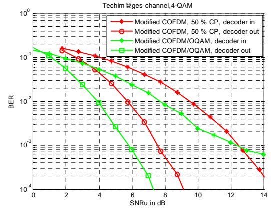
Figure 8. 4-QAM modified schemes over Techim@ges channel.
