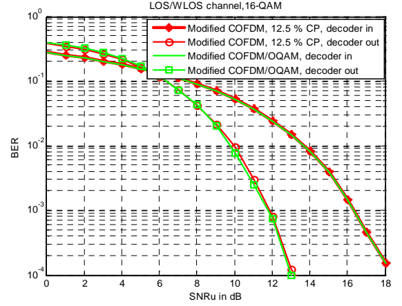
Figure 4. 16-QAM modified schemes over LOS/WLOS channel.
