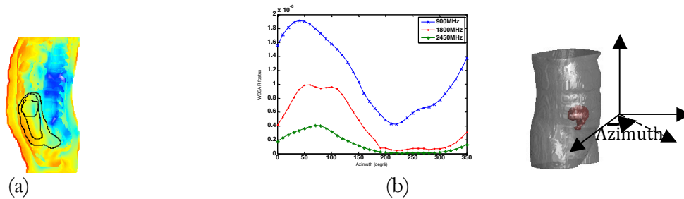
Figure 6. Normalized SAR induced by a frontal plane operating a 900 MHz wave in model 3 tissues (a) and WBSAR induced in the fetus at three different frequencies and for different incident angles in an horizontal plane (b)
