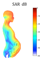
Figure 5 Model 2 exposure to frontal plane wave operating at 900 MHz.
