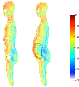
Figure 4 Normalized SAR ( color scaling in dB) induced in pregnant and non pregnant models by a frontal plane wave at 900MHz.
