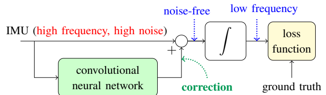
Fig. 1. Schematic illustration of the proposed method. The convolutional neural network computes gyro corrections (based on past IMU measurements) that filters undesirable errors in the raw IMU signals. We then perform open-loop time integration on the noise-free measurements for regressing low frequency errors between ground truth and estimated orientation increments.
