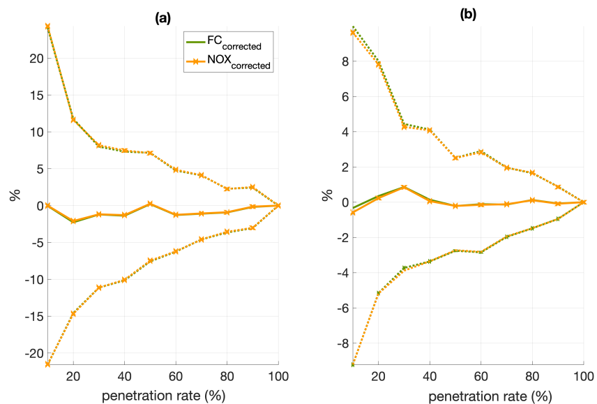
723 724 Figure 16 Relative errors on corrected emissions E(V_a) - \Delta^* , depending on the 725 penetration rate in (a) free flow conditions and (b) congested conditions, 726 assuming the total travel distance is assessed using the fishing method.
