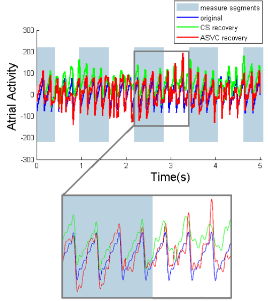
Fig. 4. Extraction of f -wave from synthetic ECG with CS (green) and ASVC (red) vs. the original fibrillatory signal (blue).
