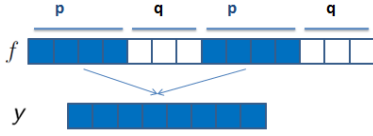
Fig. 1. (p, q) sampling scheme
