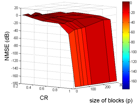
Fig. 2. NMSE (dB) of reconstructed synthetic atrial signal for block sampling for different combinations of p and CR (dB).
