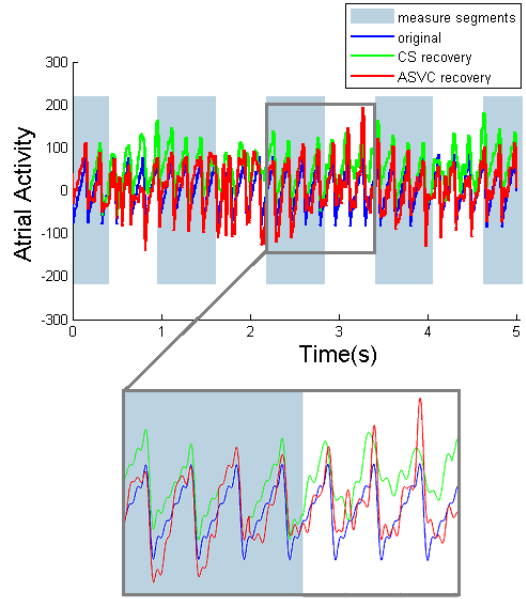
Fig. 4. Extraction of f -wave from synthetic ECG with CS (green) and ASVC (red) vs. the original fibrillatory signal (blue).
