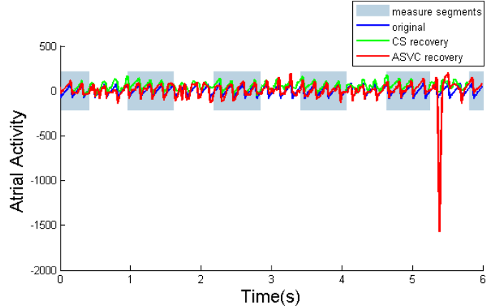
Fig. 5. Extraction of f -wave from synthetic ECG (6 s recording) with CS (green) and ASVC (red) vs. the original fibrillatory signal (blue).
