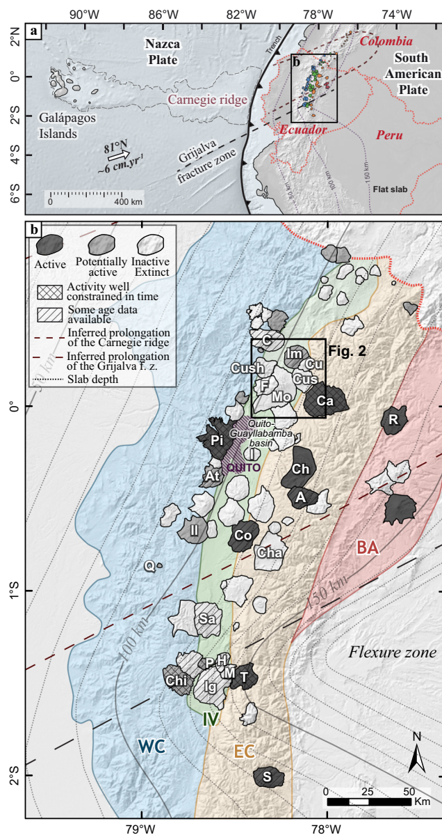
Fig. 1 a Geodynamic setting of Ecuador. White arrow indicates the direction of the Nazca plate motion relative to South America (DeMets et al. 2010). Dotted lines indicate the slab depth (purple; Yepes et al. 2016), the inferred prolongation of the Carnegie Ridge (brown; Gutscher et al. 1999a), and the Grijalva fracture zone (black). Ecuadorian Quaternary volcanoes are located in the Western and Eastern Cordilleras (blue and orange, respectively), in the Interandean Valley (green), and in the back-arc area (red). b Map of the current Ecuadorian volcanic arc. Active volcanoes (last eruption < 500 years) are represented in black, potentially active edifices (last eruption < 10 ka) in gray, and inactive or extinct Quaternary volcanoes in white (Bernard and Andrade 2011; igeppn.edu.ec ) WC: Western Cordillera (blue field); IV: Interandean Valley (green); EC: Eastern Cordillera (orange); BA: back-arc area (red). Notable and mentioned in text volcanoes: A: Antisana; At: Atacazo; Ca: Cayambe; Ch: Chacana; Cha: Chalupas; Chi: Chimborazo; C: Cotacachi; Co: Cotopaxi; Cu: Cubilche; Cus: Cusín; Cush: Cushnirumi; F: Fuya Fuya; H: Huisla; Ig: Iguálata; I: Ilaló; Il: Iliniza; Im: Imbabura; Mo: Mojanda; M: Mulmul; Pi: Pichincha; P: Puñalica; R: Reventador; Q: Quilotoa; Sa: Sagoatoa; S: Sangay; T: Tungurahua
