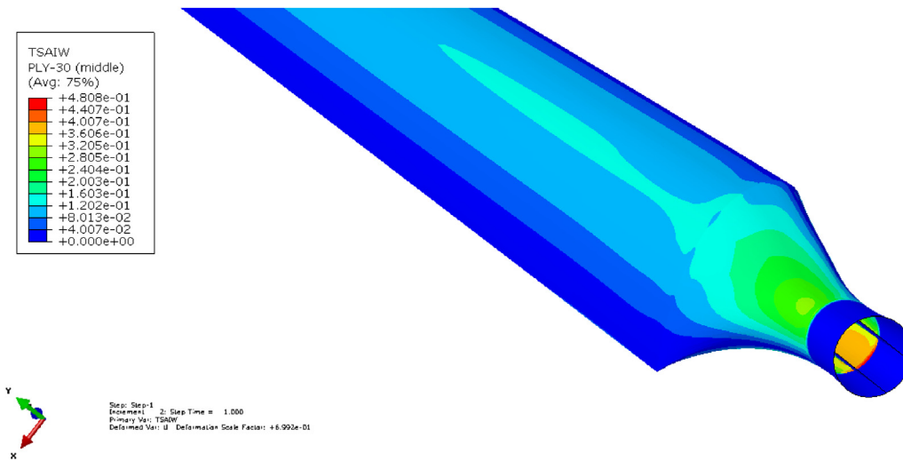
Fig. 14. Tsai-Wu failure criterion value of 45° ply at Type-1 configuration.
