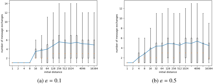
Fig. 15: Two players moving, random walk, 3D: M depending on initial distance
