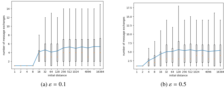
Fig. 12: Two players moving, random walk, 2D: M depending on initial distance
