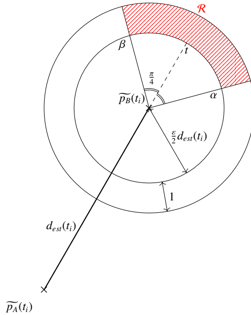
Fig. 4: Representation of the points corresponding to an increasing jump
