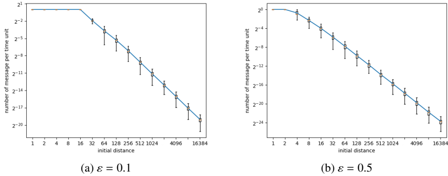
Fig. 14: Two players moving, random walk, 2D: messages per time unit with \mathcal{A}_c
