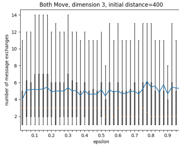
Fig. 18: Two players moving, random walk, 3D: M depending on \epsilon , for d_0 = 400
