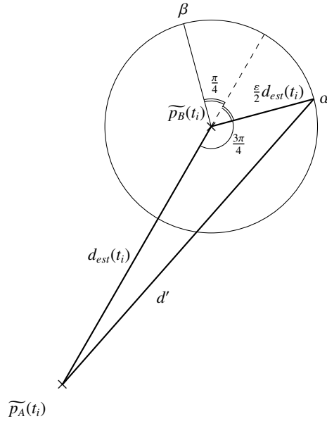
Fig. 6: Representation of the different values used to measure an increasing jump
