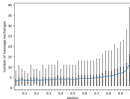
Fig. 9: One player moving, random walk, 1D: value of M depending on \epsilon , for d_0 = 400
