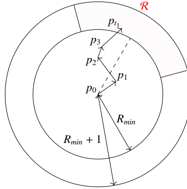
Fig. 5: Representation of the values used in proof of Lemma 11
