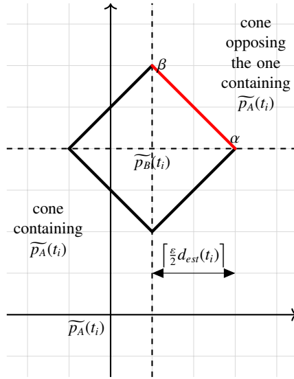
Fig. 2: Two-dimensional example: one of the outer bounds of I_{lc}^+ is always sufficiently far away from \widetilde{p}_A(t_i)
