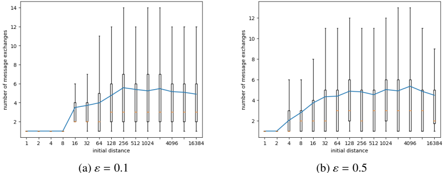
Fig. 16: Two players moving, random walk, 3D: M depending on initial distance
