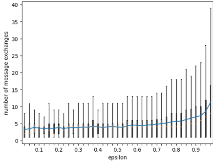
Fig. 9: One player moving, random walk, 1D: value of M depending on \epsilon , for d_0 = 400
