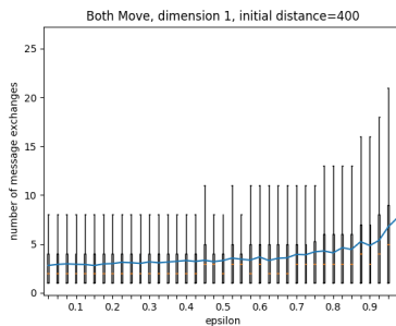
Fig. 12: Two players moving, random walk, 1D: M depending on \epsilon , for d_0 = 400
