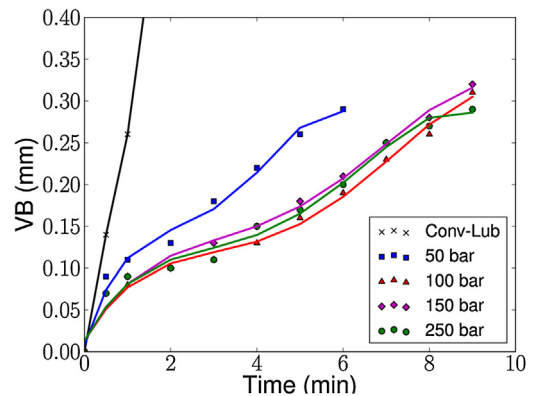
Fig. 11. Flank wear evolution, V_c = 88 m/min.
