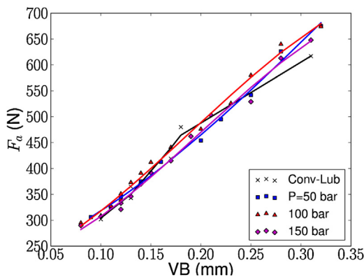
Fig. 10. Evolution of the axial force as a function of flank wear ( V_c = 75 m/min).
