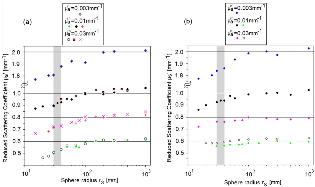
Fig. 3. Retrieved reduced scattering coefficient \mu_s' , for an apple assimilated to a sphere with different radii. The departure from the horizontal continuous lines (true values: 0.6, 0.8, 1 and 2 \text{mm}^{-1} ) represents errors involved in the estimates calculated with the Monte Carlo code. (a) Use of an approximated analytical method to assess \mu_s' . (b) Use of a Levenberg–Marquardt fitting algorithm.
