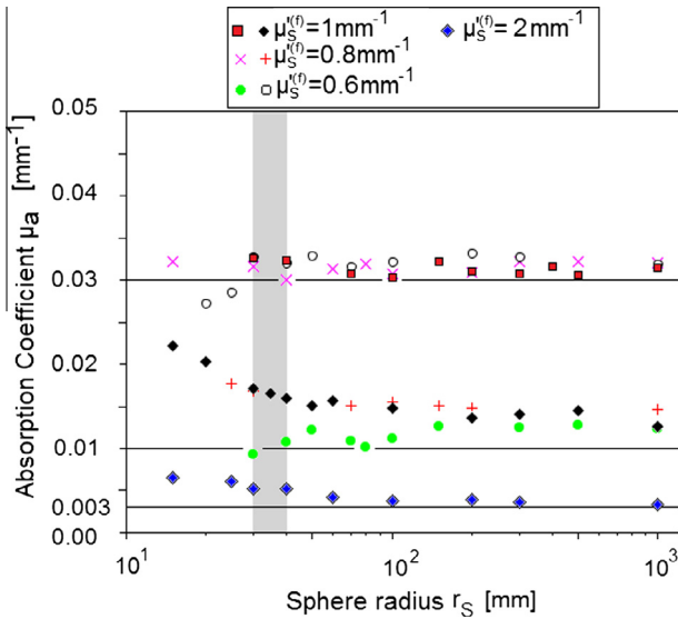
Fig. 4. Retrieved absorption coefficient \mu_a , for a homogeneous sphere with different radii using prior \mu_s' information to initiate a Levenberg–Marquardt algorithm. Monte Carlo data were generated with \mu_a^{(t)} = 0.003, 0.01, 0.03 \text{ mm}^{-1} and \mu_s'^{(t)} = 0.6, 0.8, 1 and 2 \text{ mm}^{-1} . The departure from the horizontal continuous lines represents error in the estimates.
