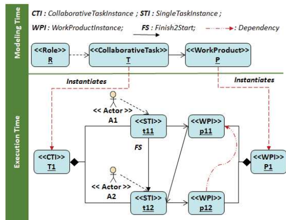
Figure 4: Pattern SEQ-INSTANCES-COP for a collaborative task T .
