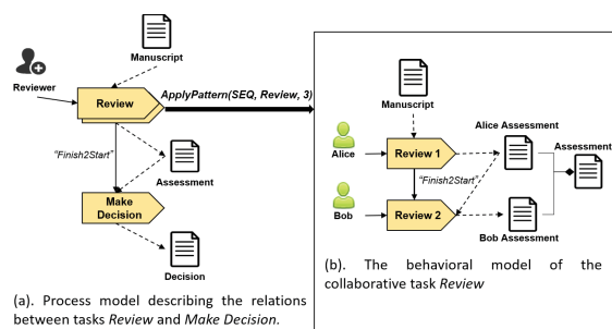
Figure 5: Application of SEQ-INSTANCES-COP to define the relations among the task Review ’s instances.
