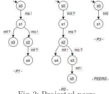
Fig. 2: Projected peers.
