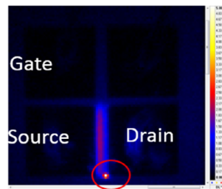
Fig. 11. Amplitude image with lock-in thermography after HBM-ESD stress on SiC MESFET.
