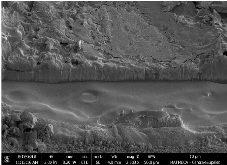
Fig. 15. Zoom on failure in SiC vertical diode.
