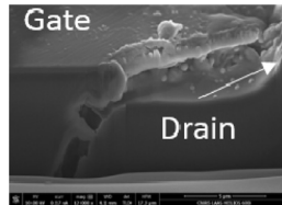
Fig. 13. SEM image after FIB on a failure in SiC MESFET after ESD [7].
