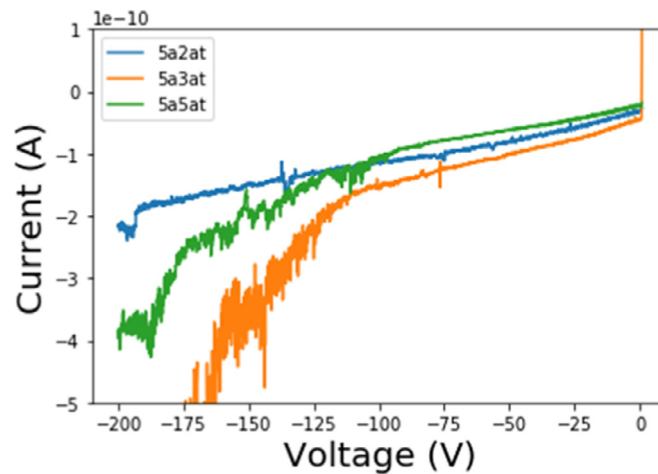
Fig. 9. I-V for three vertical diodes.
