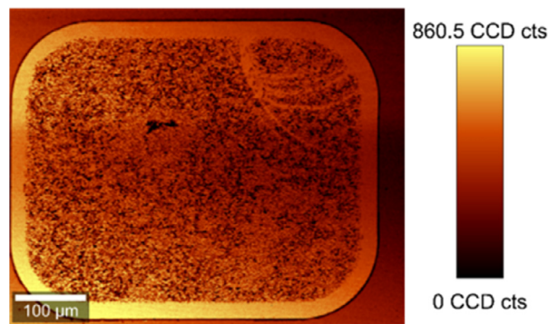
Fig. 19. Micro-Raman mapping of the Sic integrated intensity.
