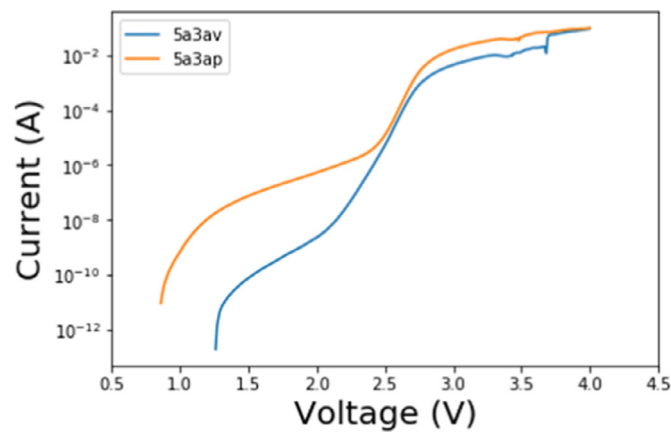
Fig. 6. I-V in semilogy for SiC vertical diode before failure (5av2) and after (5ap2).
