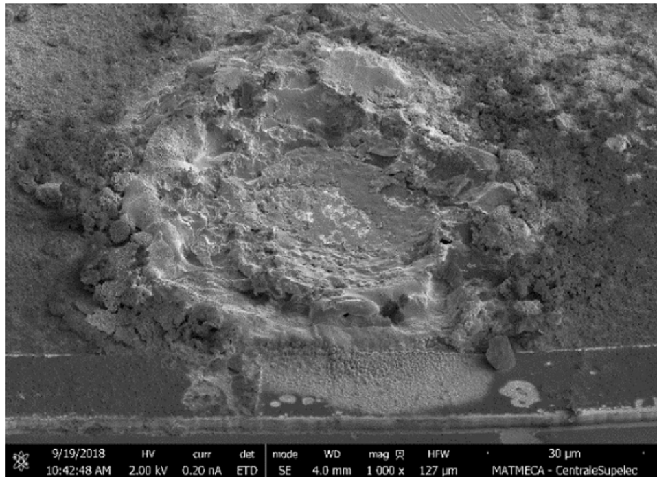
Fig. 14. SEM Image after FIB on a failure after high voltage applied on SiC vertical diode.
