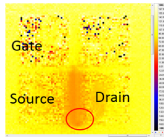
Fig. 12. Phase image with lock-in thermography after HBM-ESD stress on SiC MESFET.
