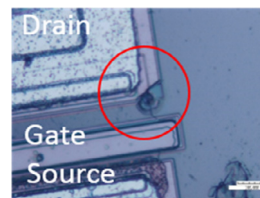
Fig. 10. Failure at the MESFET corner after HBM-ESD stress.
