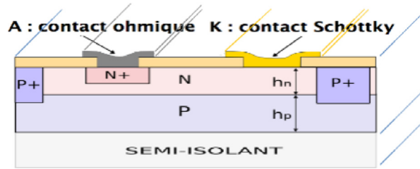
Fig. 2. Transversal section of lateral Schottky diode.
