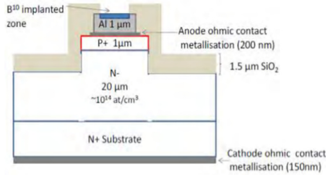
Fig. 1. Transversal section of vertical SiC diode.
