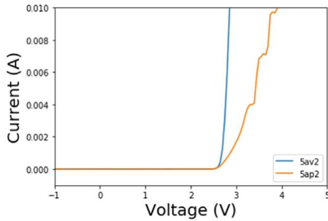
Fig. 5. I-V for SiC vertical diode before failure (5av2) and after (5ap2).
