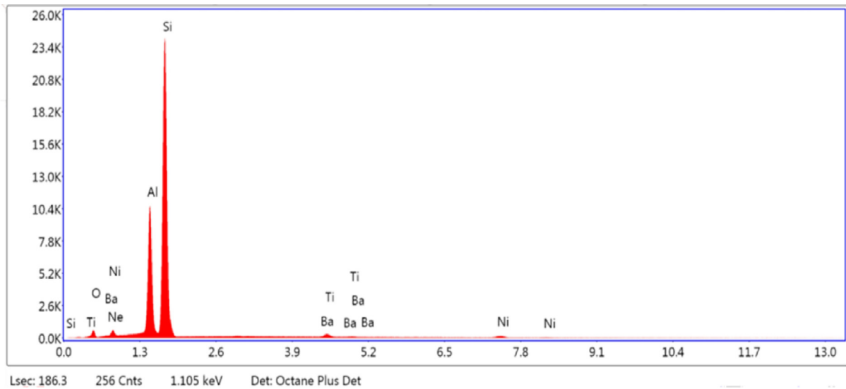
Fig. 17. EDX of SiC vertical diode before failure.
