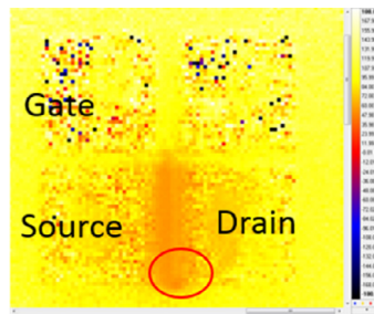
Fig. 12. Phase image with lock-in thermography after HBM-ESD stress on SiC MESFET.
