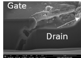
Fig. 13. SEM image after FIB on a failure in SiC MESFET after ESD [7].
