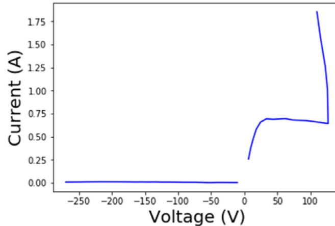
Fig. 4. I-V after HBM-ESD stress on SiC lateral diode.
