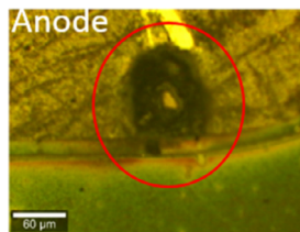
Fig. 8. Optical microscopy after high voltage failure on the corner of the device.
