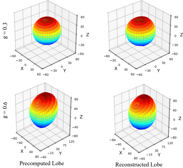
Fig. 4. Comparison between the lobe simulated using the Monte Carlo method and the one reconstructed by our neural network. Material: Bumpy-sphere, g = 0.3 and g = 0.6 , lobe position (4.8, 4.8).
