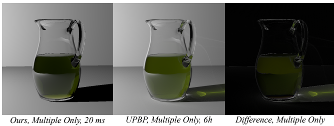
Fig. 19. Comparison between our method and references on a medium with a low albedo (Oil). On this material, low-order scattering effects dominate. Our method tends to underestimate multiple scattering, due to the inaccuracy of neural network representation for extremely small values caused by the low albedo in the media.
