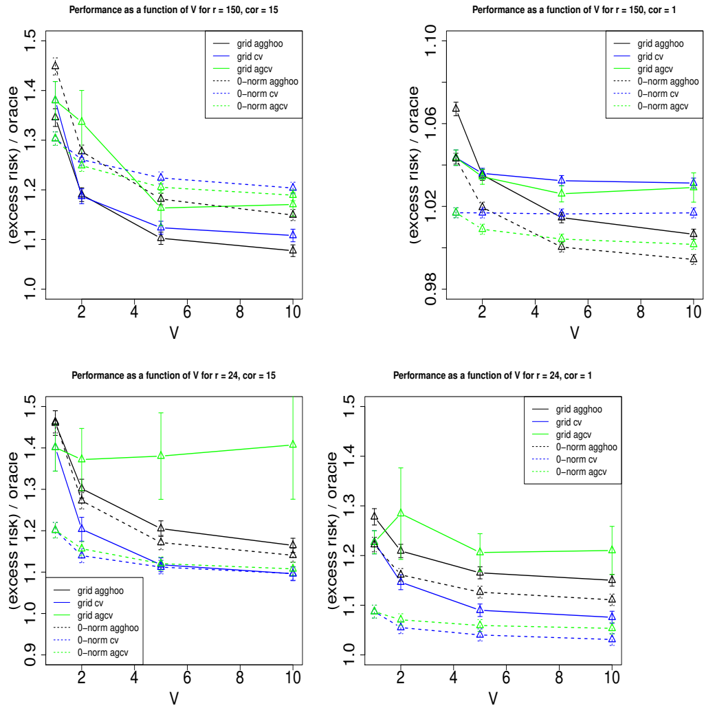
Figure 1: Performance relative to the oracle, as a function of V
