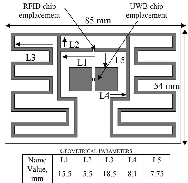
Figure 1: Tag antennas
